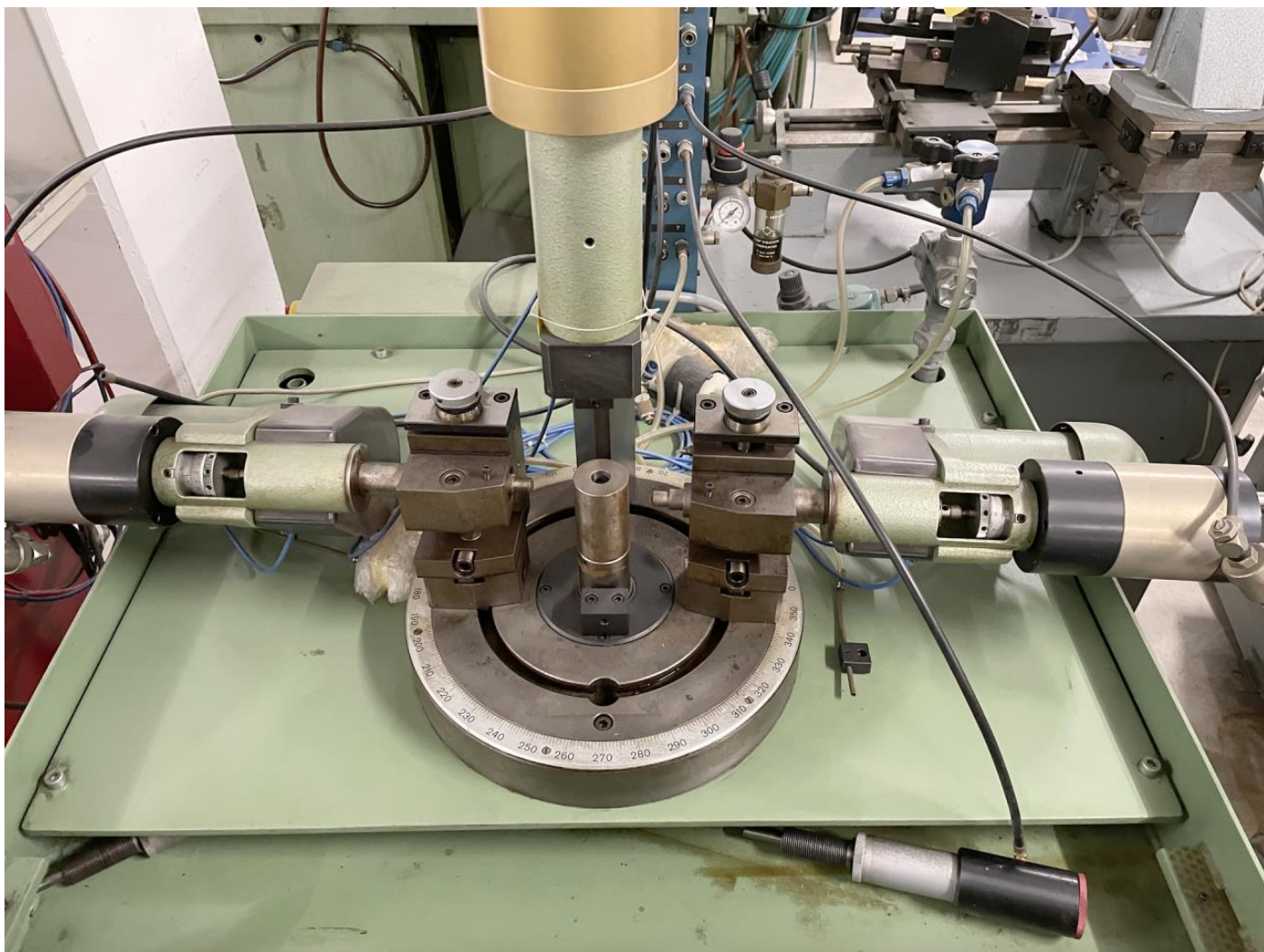
Cast-iron base
