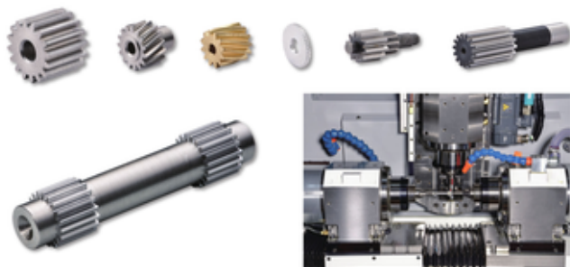
Workpiece
